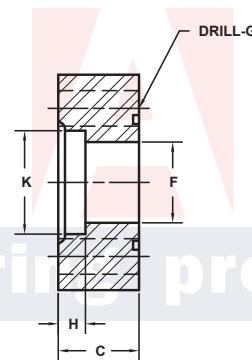
Model 6531 / 6535
