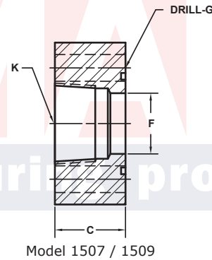
O-Ring Style
